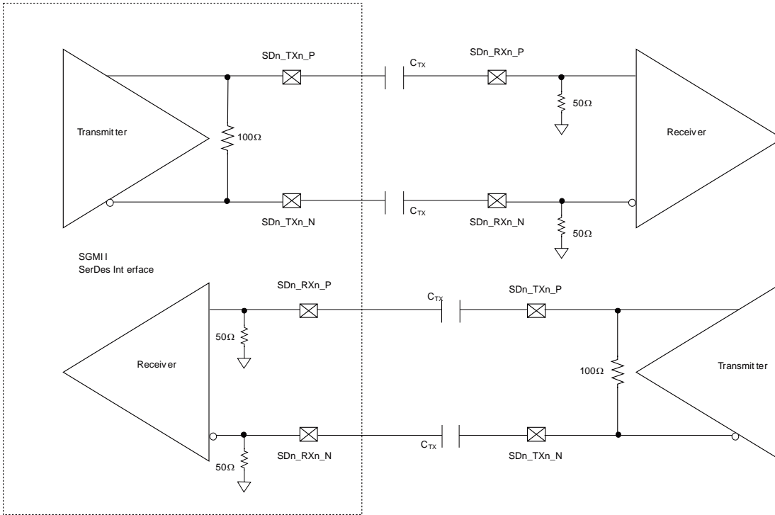
Figure 14. 4-wire AC-coupled SGMII serial link connection example
