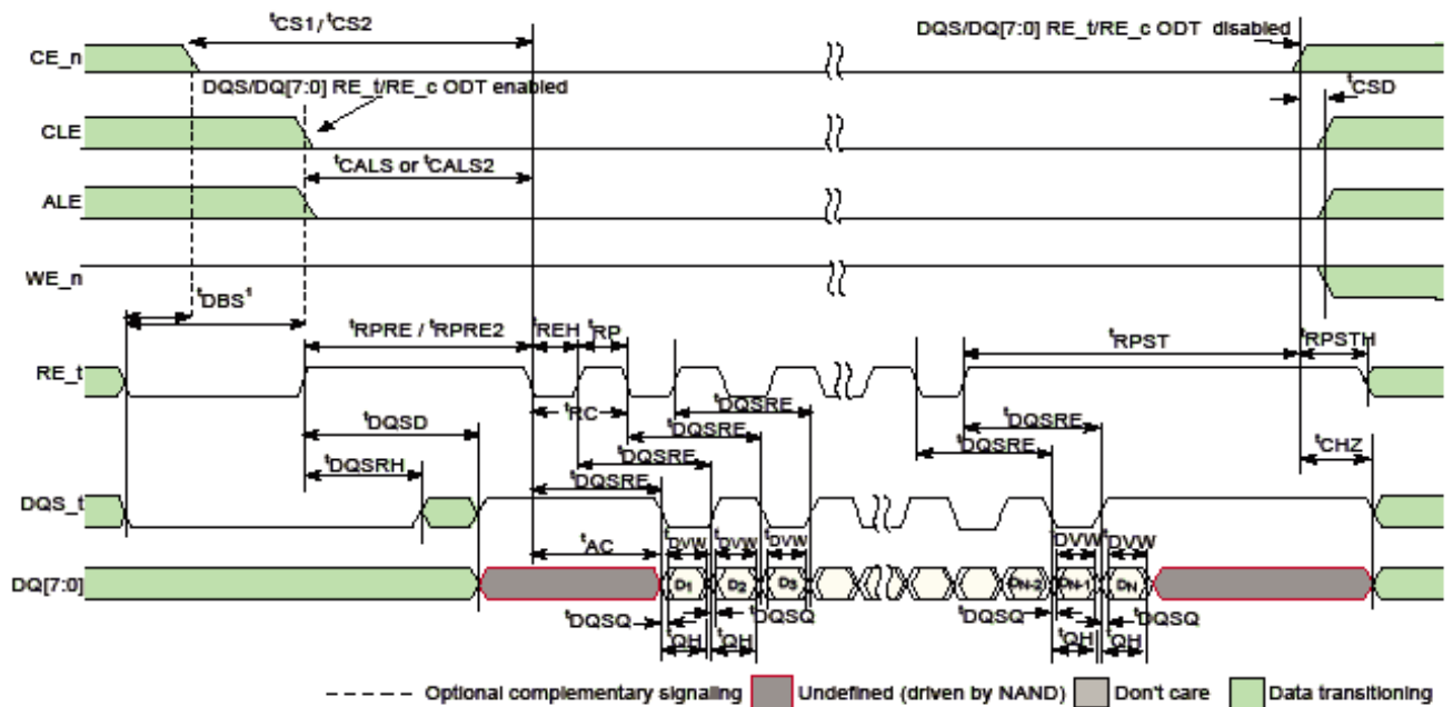
Figure 50. Read cycle
