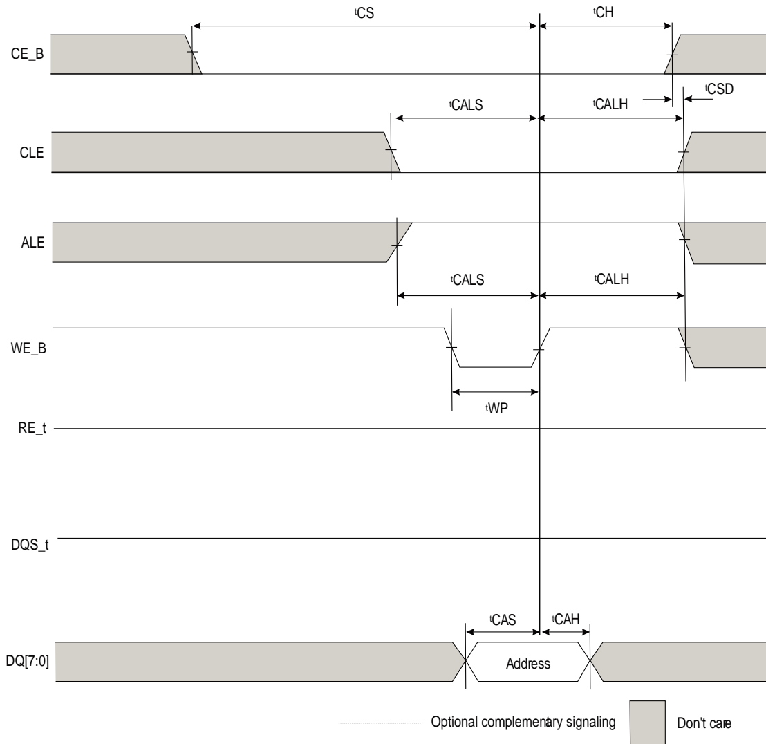
Figure 48. Address cycle
