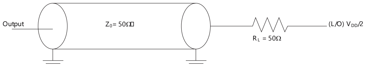
Figure 76. GPIO AC test load
