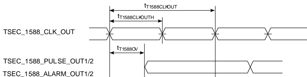
Figure 23. IEEE 1588 output AC timing
