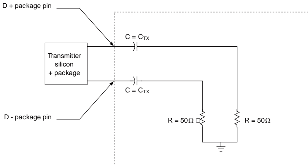
Figure 86. Test and measurement load
