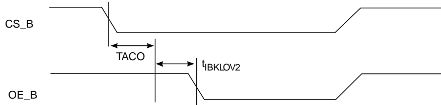
Figure 30. IFC-NOR interface output AC timings
