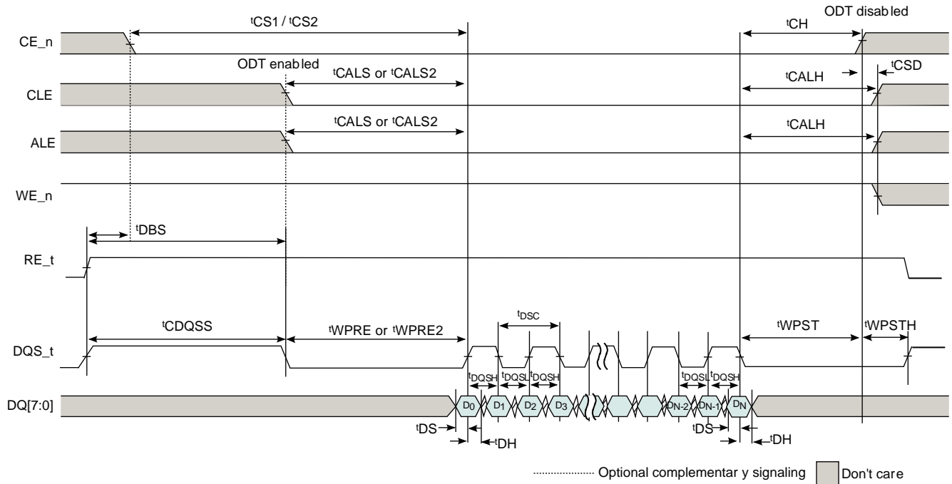
Figure 49. Write cycle
